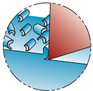
der Reißspan discontinuous chip
